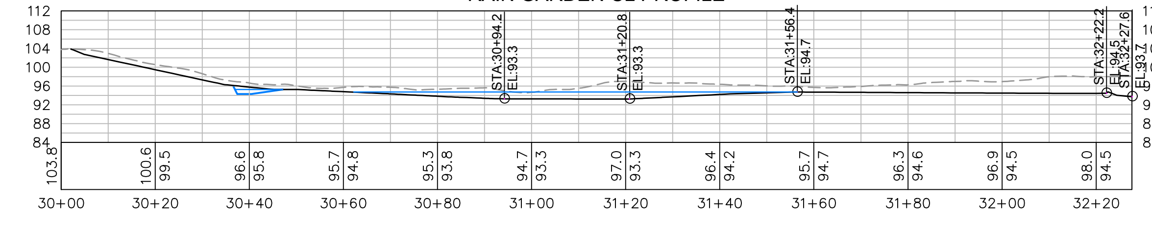
RAIN GARDEN CL PROFILE
